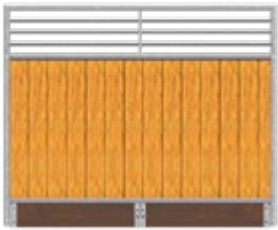
Standard plus fence elements: Height 1,60 m
